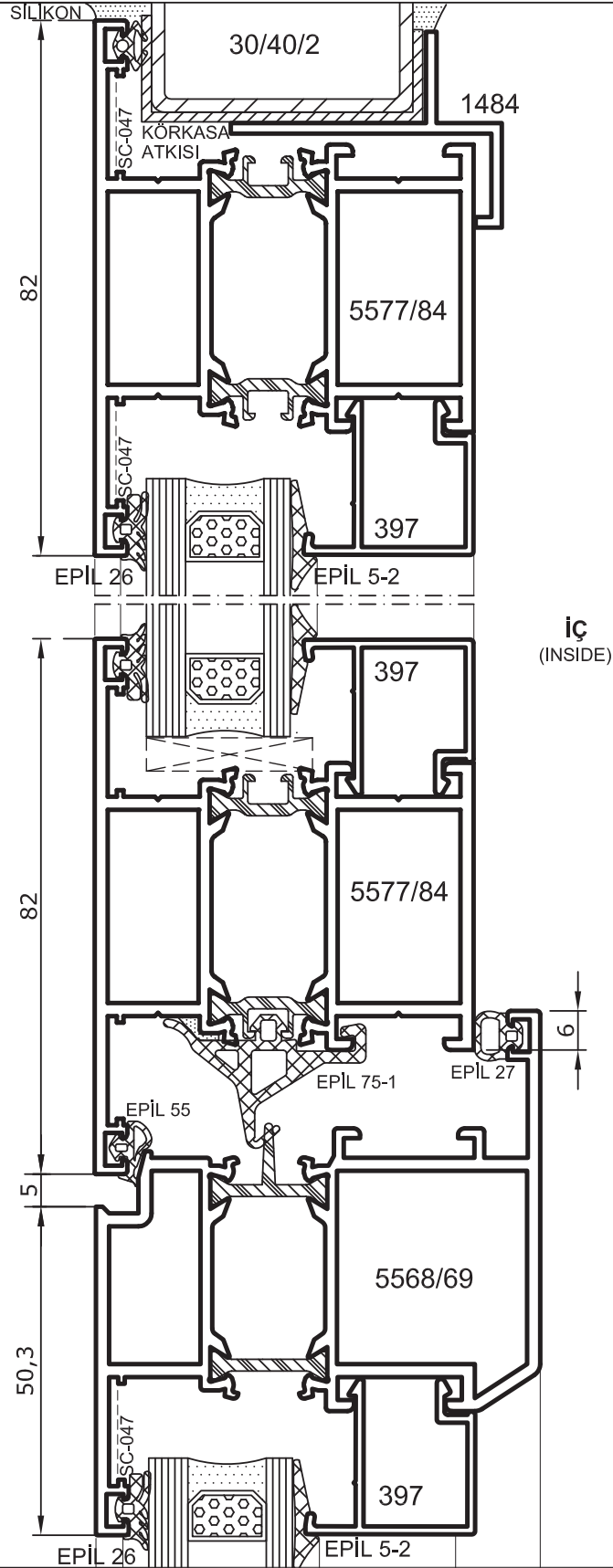
Detay Detail 5
