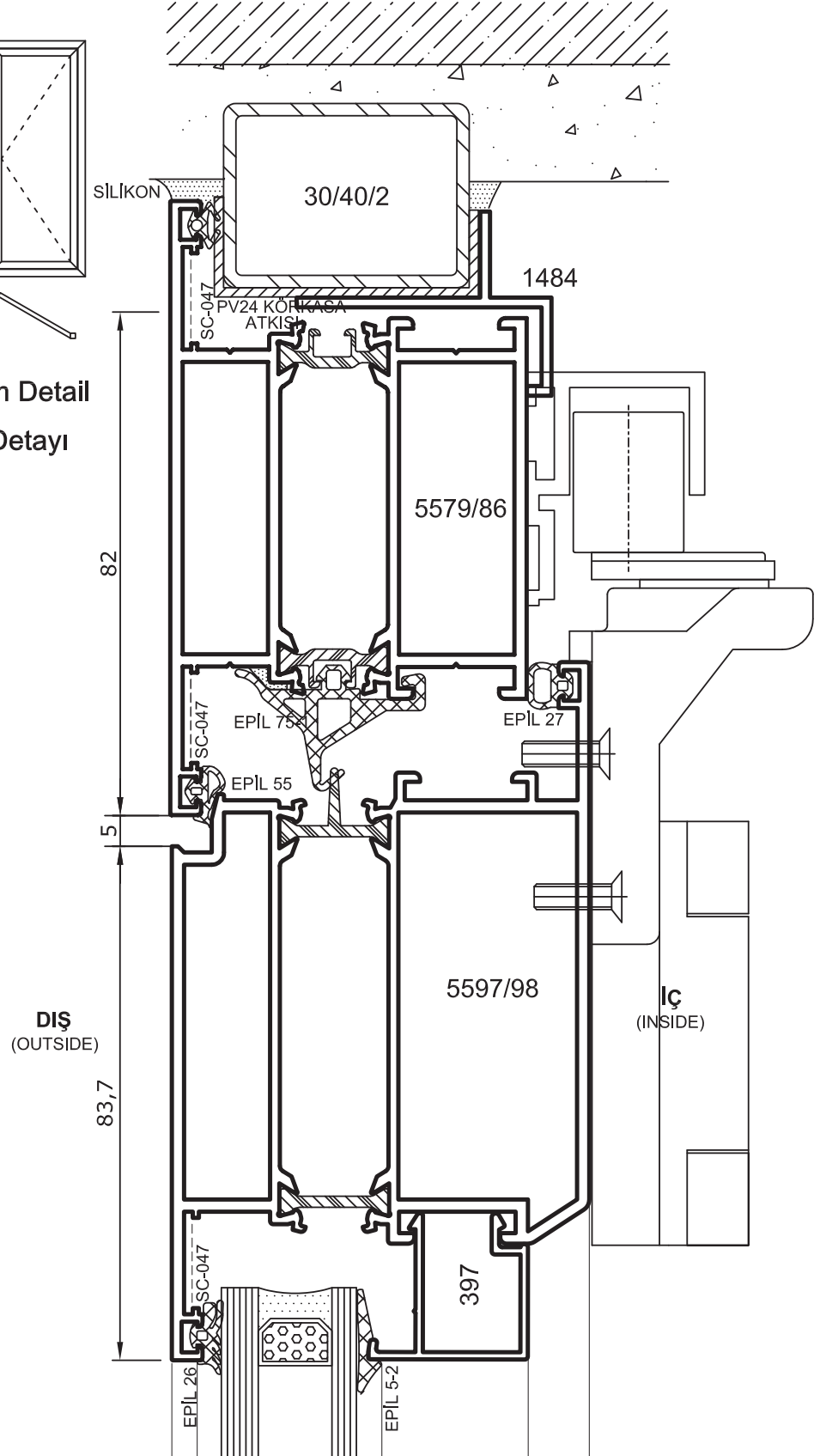
Detay Detail 6
