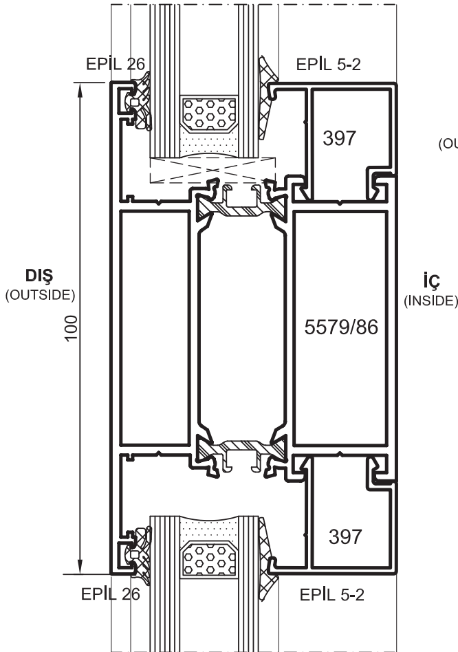
Detay Detail 4
