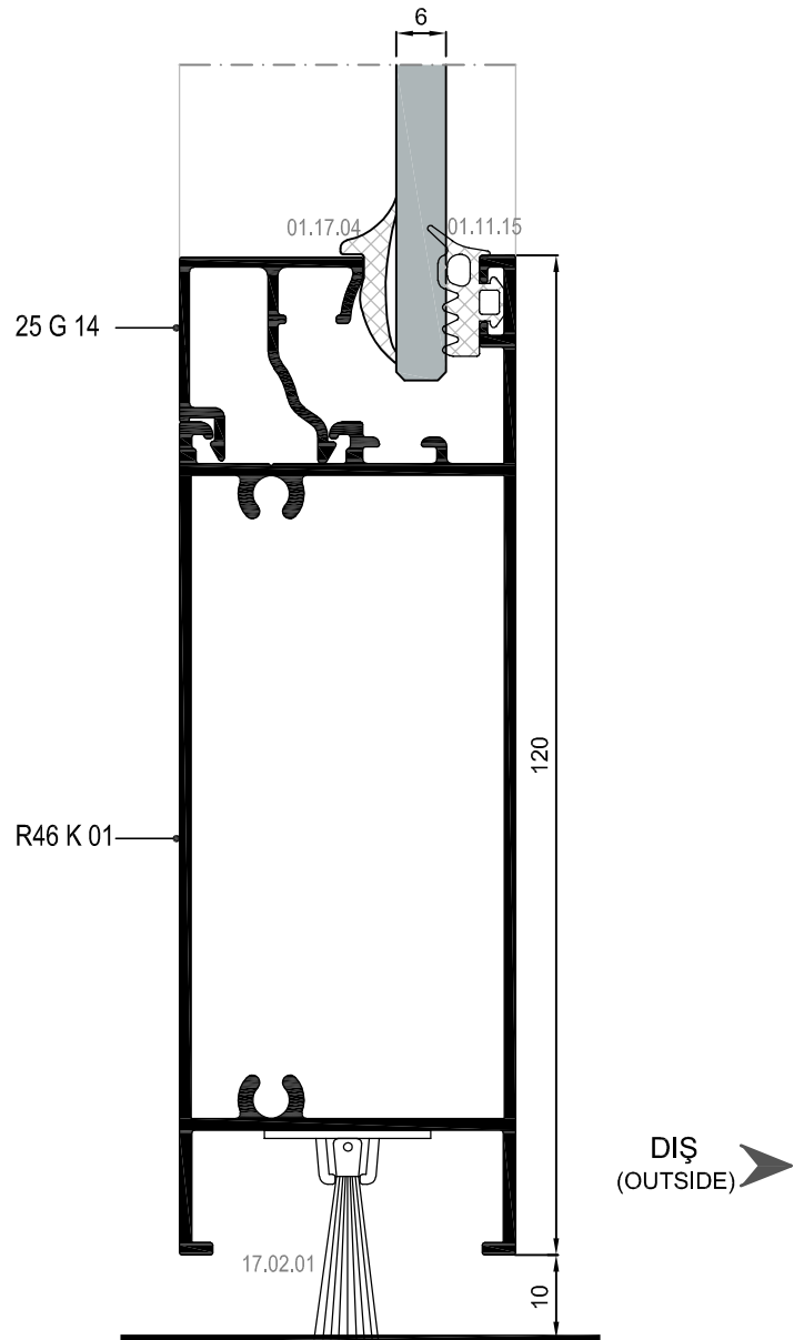
16 DETAYI DETAIL
