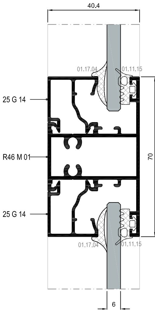
15 DETAYI DETAIL
